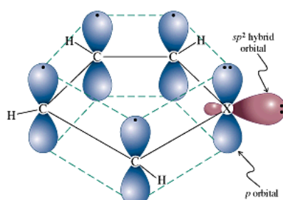
Furan (X = O) Thiophene (X = S)
