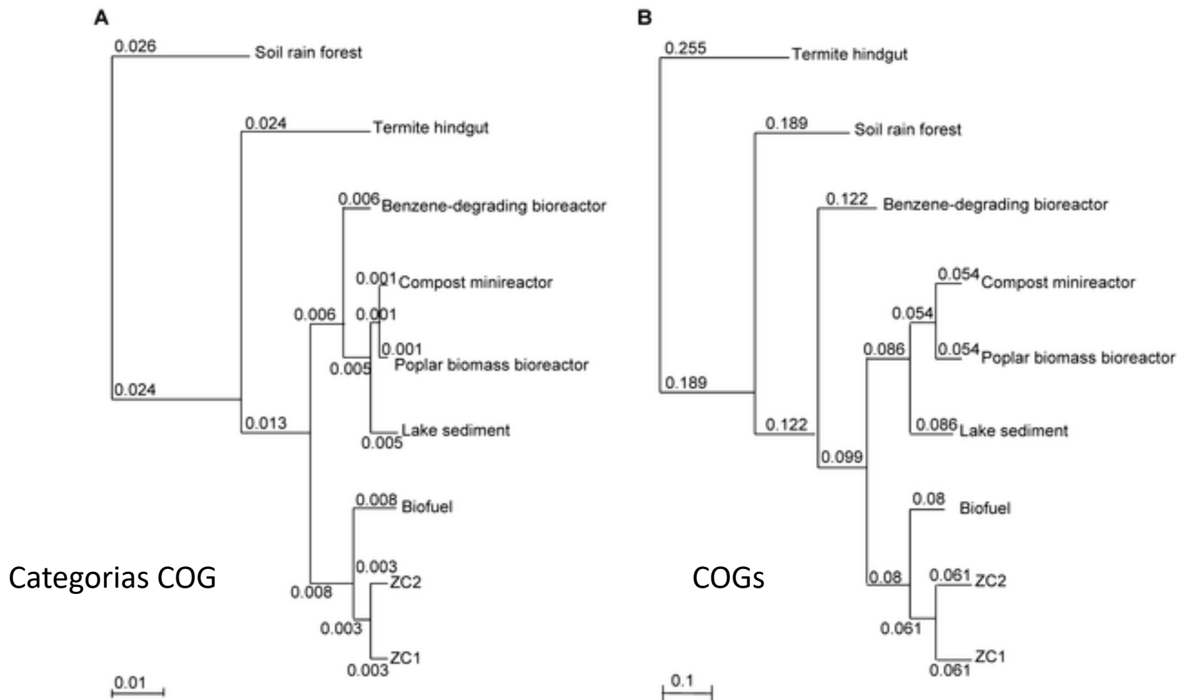
Figure 8. Hierarchical clustering of functional gene groups of ZC1 and ZC2 and seven public metagenomes.
