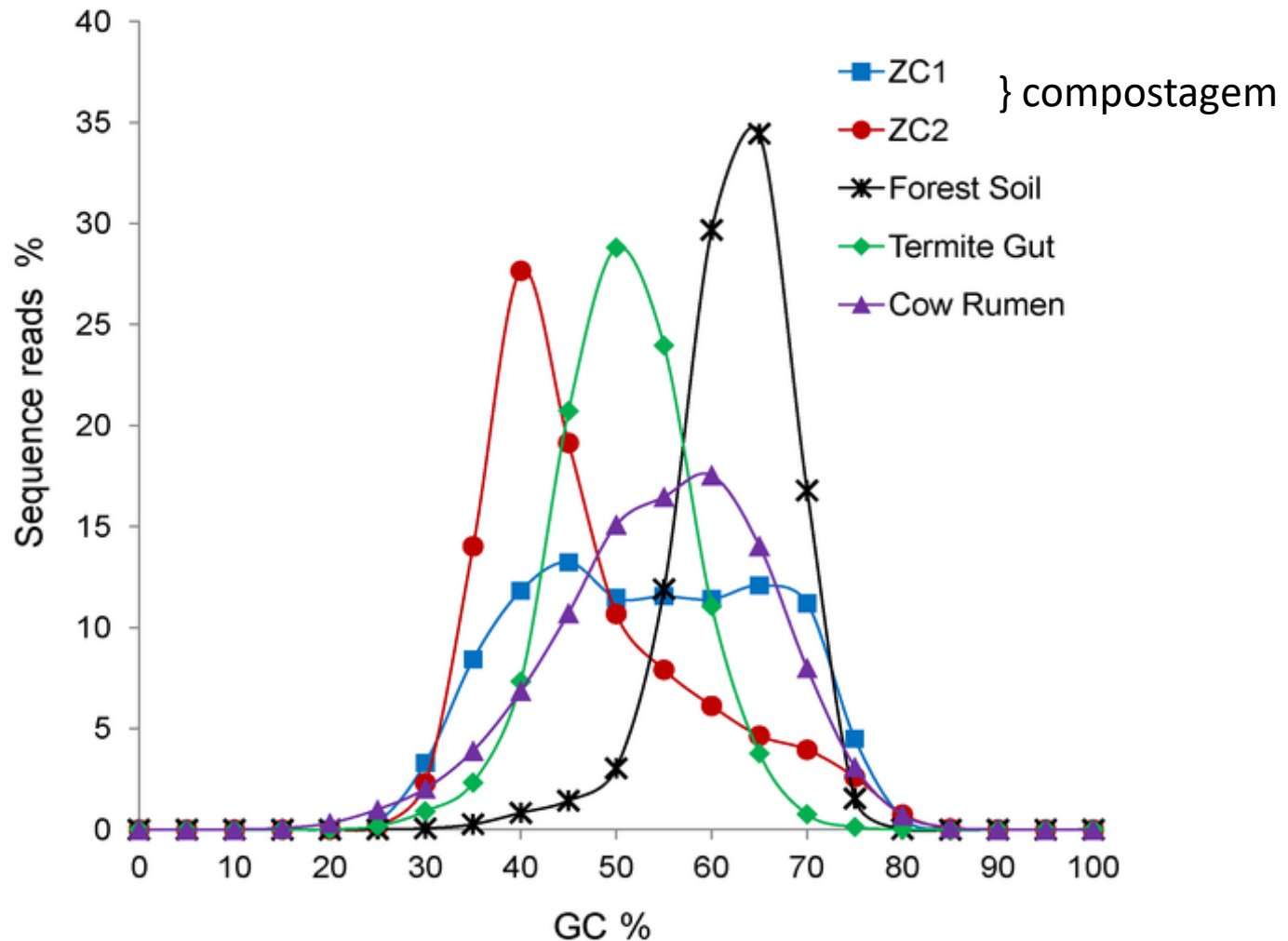
Figure 1. Distribution of the GC content percentage for ZC1 and ZC2 compared with selected metagenomes.
